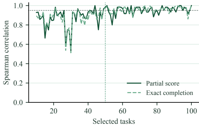
(c) OSWorld ranking
