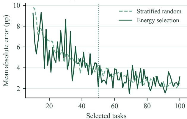
(c) OSWorld ranking
